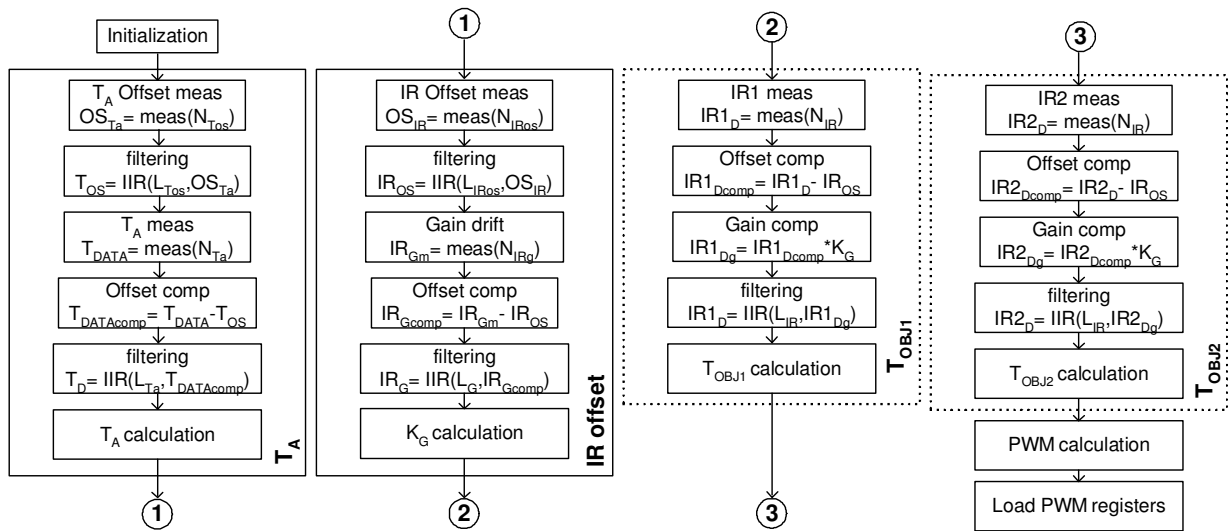
Figure 20: Software flow
