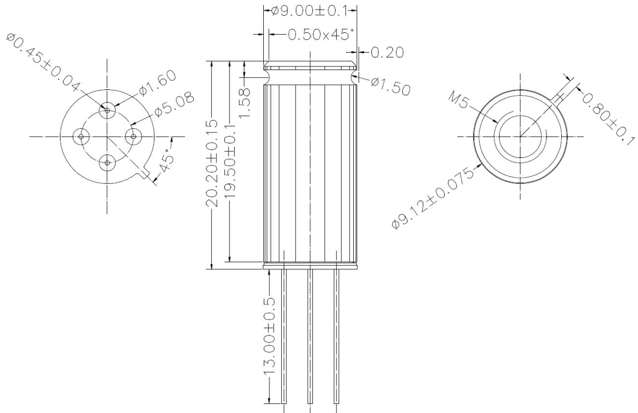
Figure 45: MLX90614xCI package
