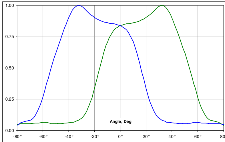
Figure 29: Typical FOV of MLX90614xBA
