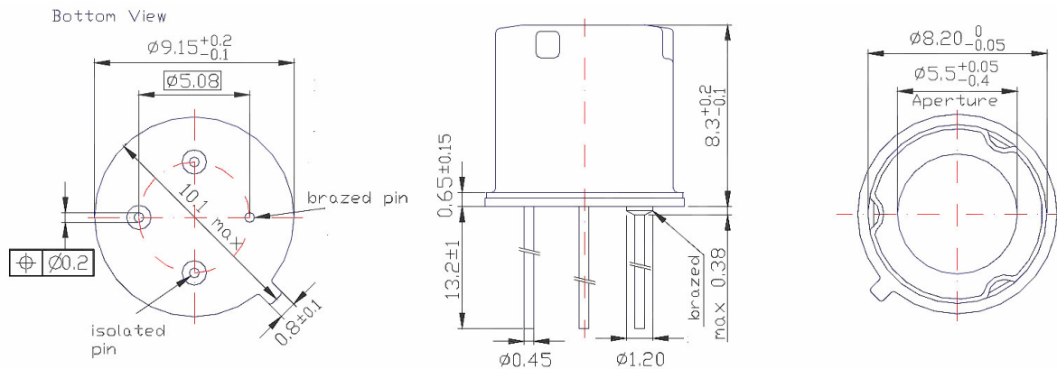
Figure 44: MLX90614xCH package
