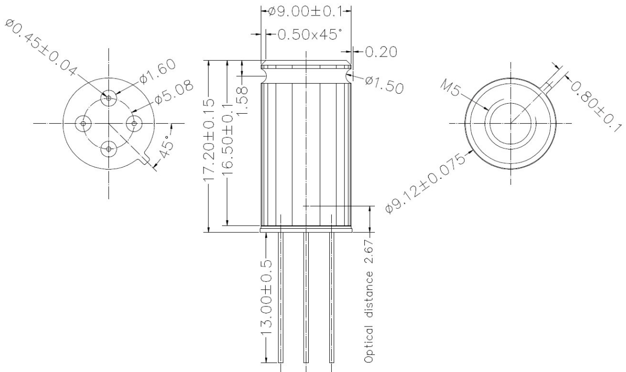
Figure 43: MLX90614xCF package
